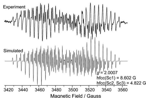
Figure 4. Experimental and simulated ESR spectra of the \text{Sc}_3\text{C}_2\text{@C}_{80} fulleropyrrolidine monoadduct.
