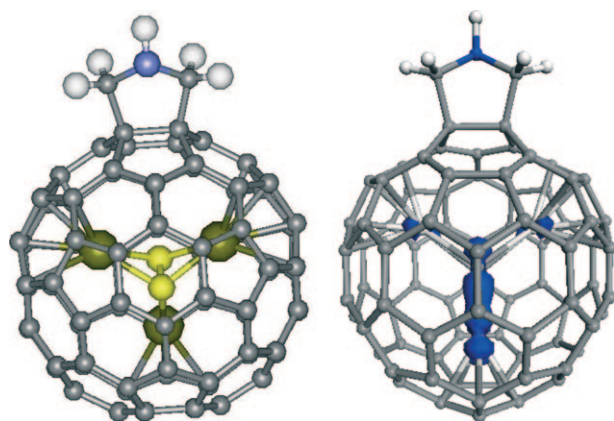
Figure 3. Optimized structure (left; N blue, Sc yellow, C gray, H white) and calculated spin density distribution (right) of the \text{Sc}_3\text{C}_2\text{@C}_{80} fulleropyrrolidine monoadduct.
